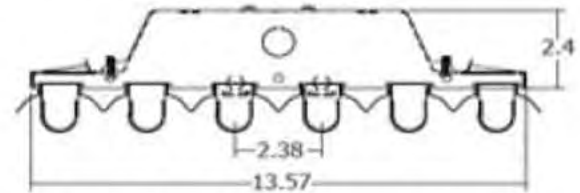
6-Lamp end view showing reflector configuration and lamp location
